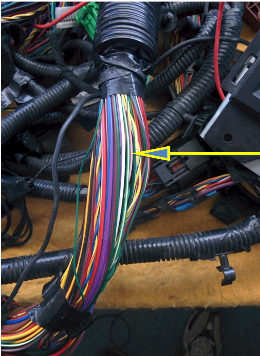
Twisted CAN pair found in loom
